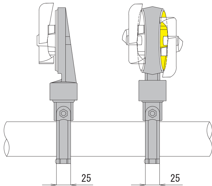
ATD-100S (片面)
